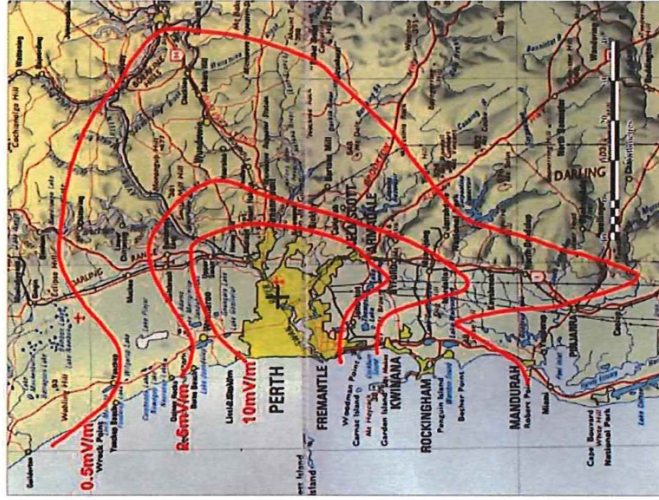
6RPH Belmont - Coverage Contours Based on Field Strength Survey May 2004
